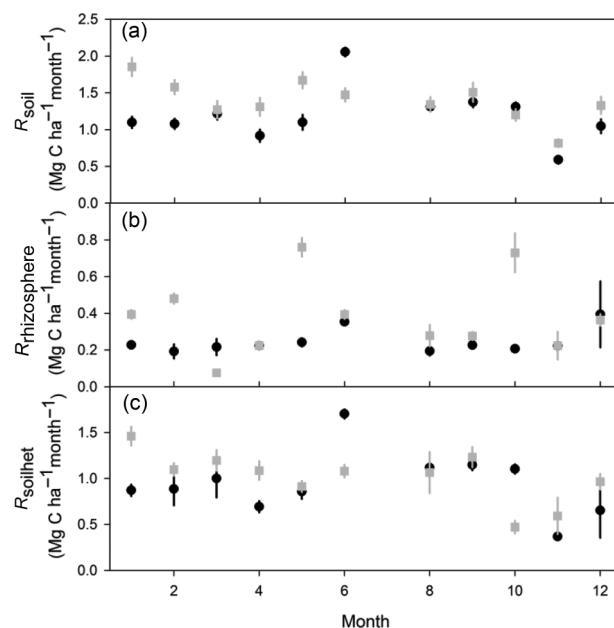
Figure 5. (a) Total soil respiration in units of \text{Mg C ha}^{-1} \text{ month}^{-1} from 25 collars measured monthly. (b) rhizosphere respiration; (c) heterotrophic soil respiration. Tower plot (black circles) and the terra preta plot (grey squares) in the Caxiuanã National Forest Reserve, eastern Amazonia, Brazil. Error bars are standard errors.
